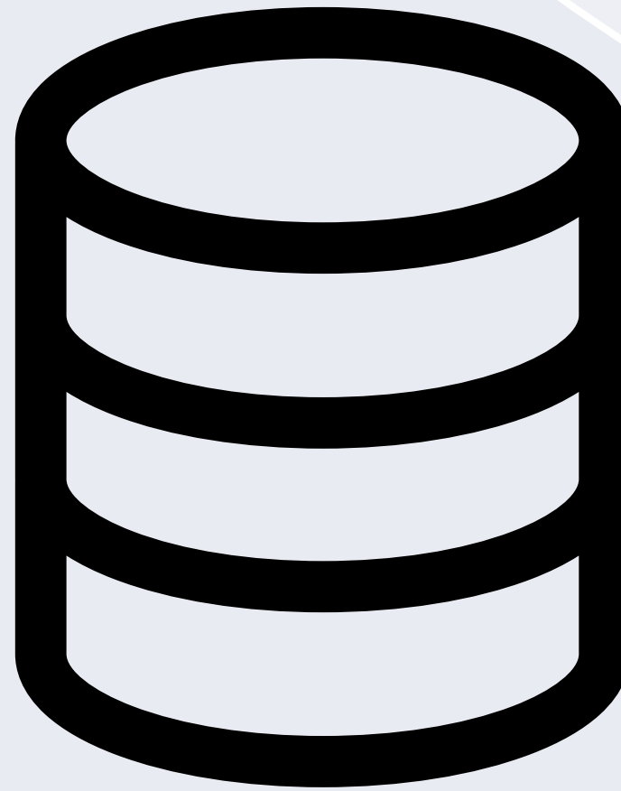
PostgreSQL (pgvector)
